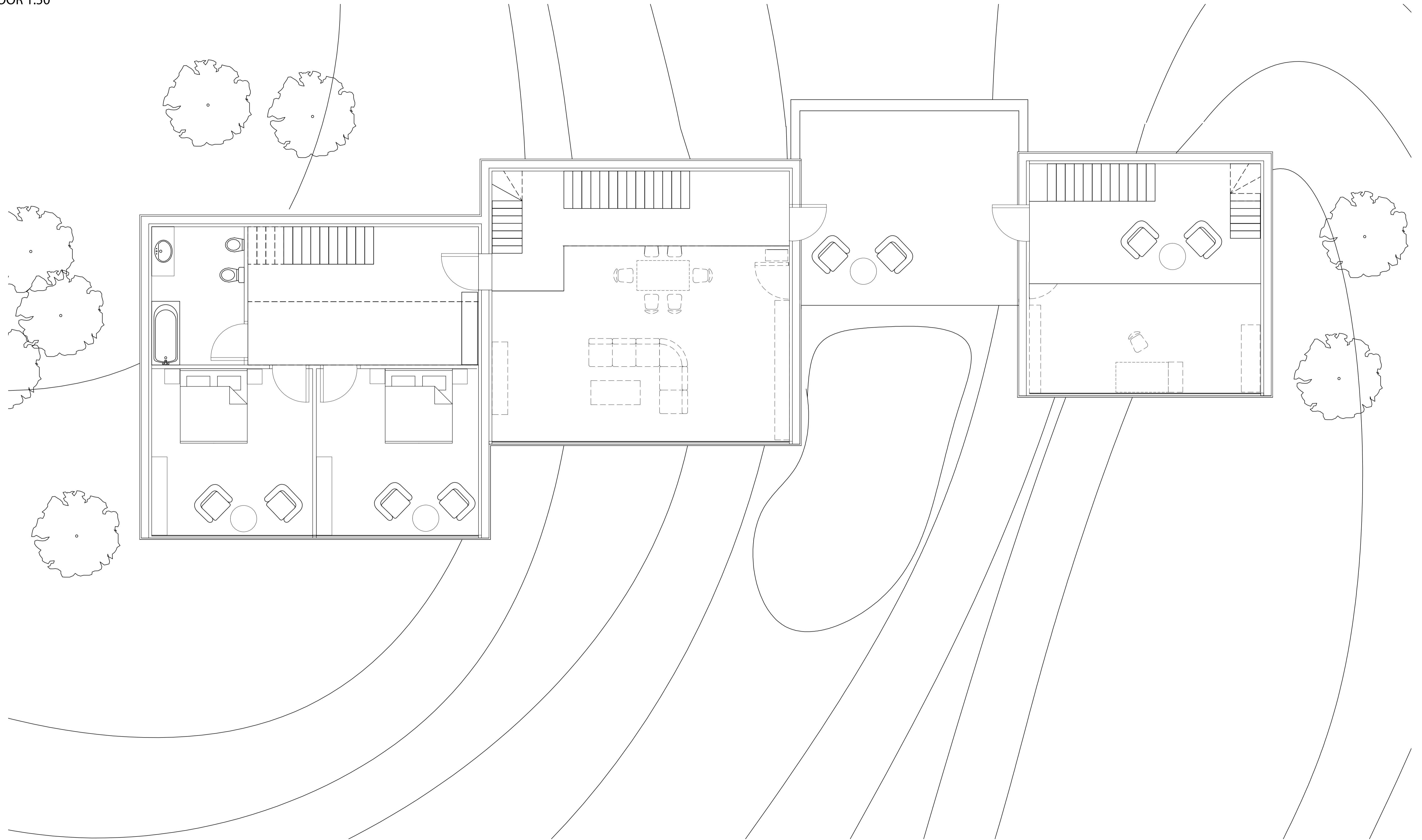
FIRST FLOOR 1:50
