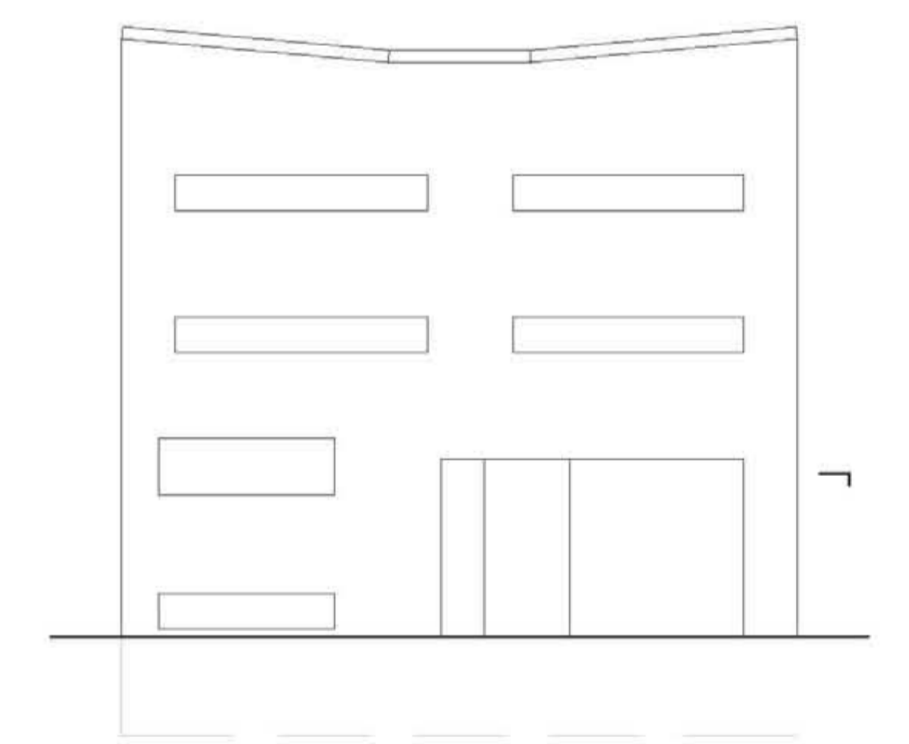
TYPE A NORTH ELEVATION scale 1:100
