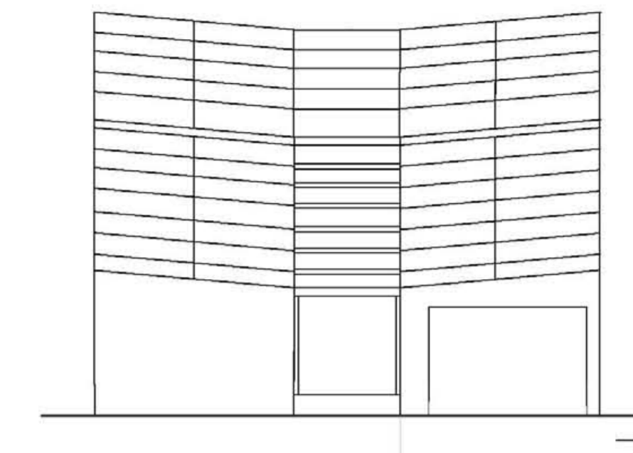
TYPE B SOUTH ELEVATION scale 1:100
