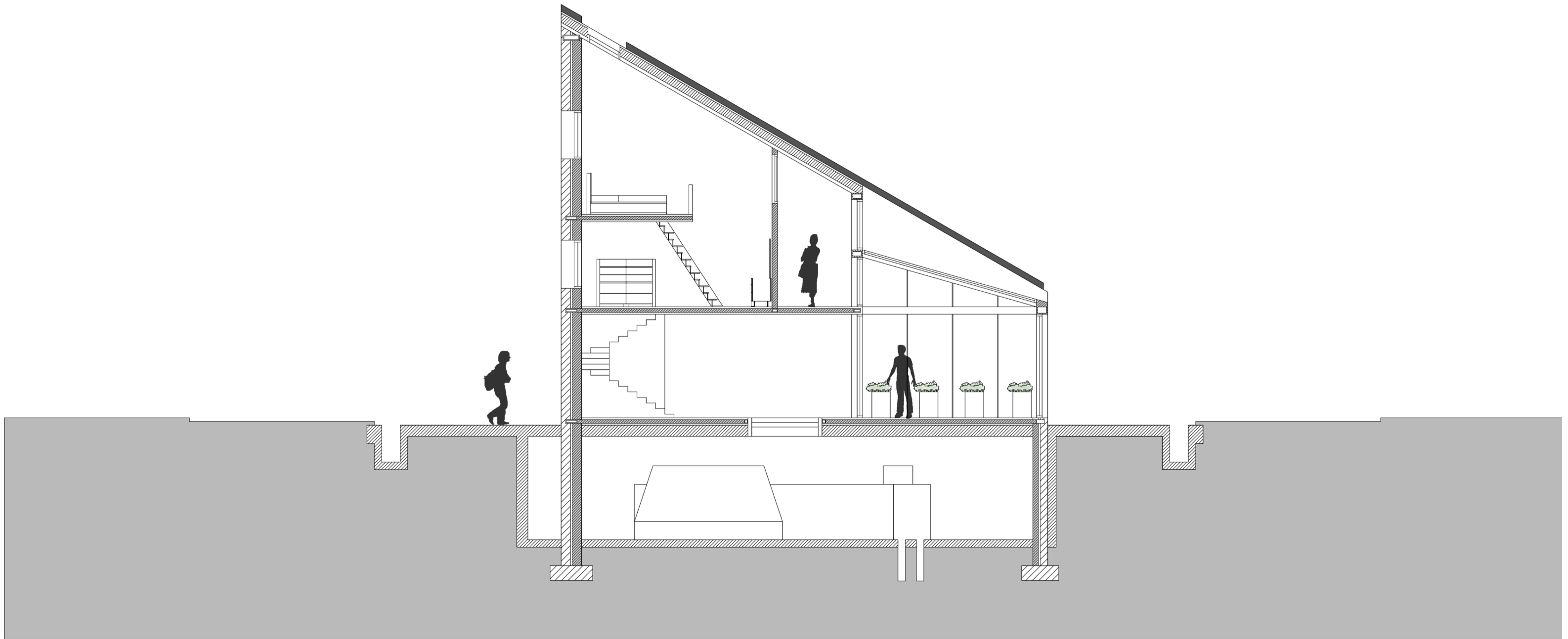
HOUSE SECTION
