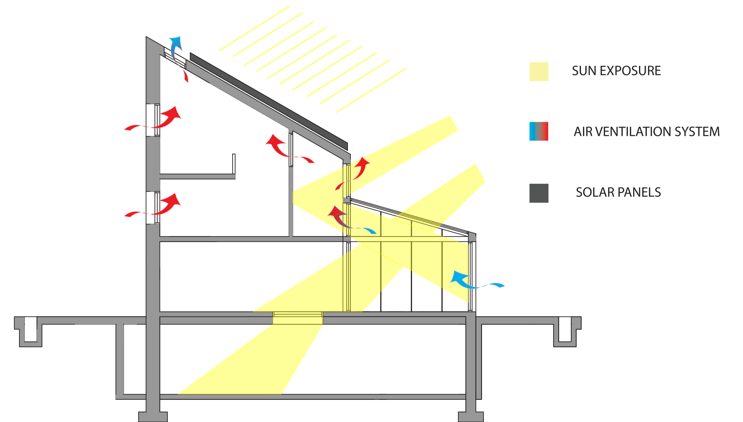
SUN EXPOSURE AND AIR VENTILATION DIAGRAM
