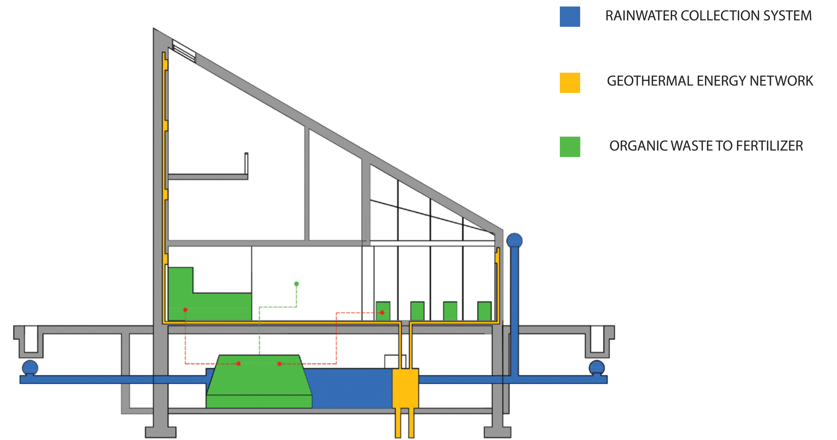
PERFORMANCE DIAGRAM
