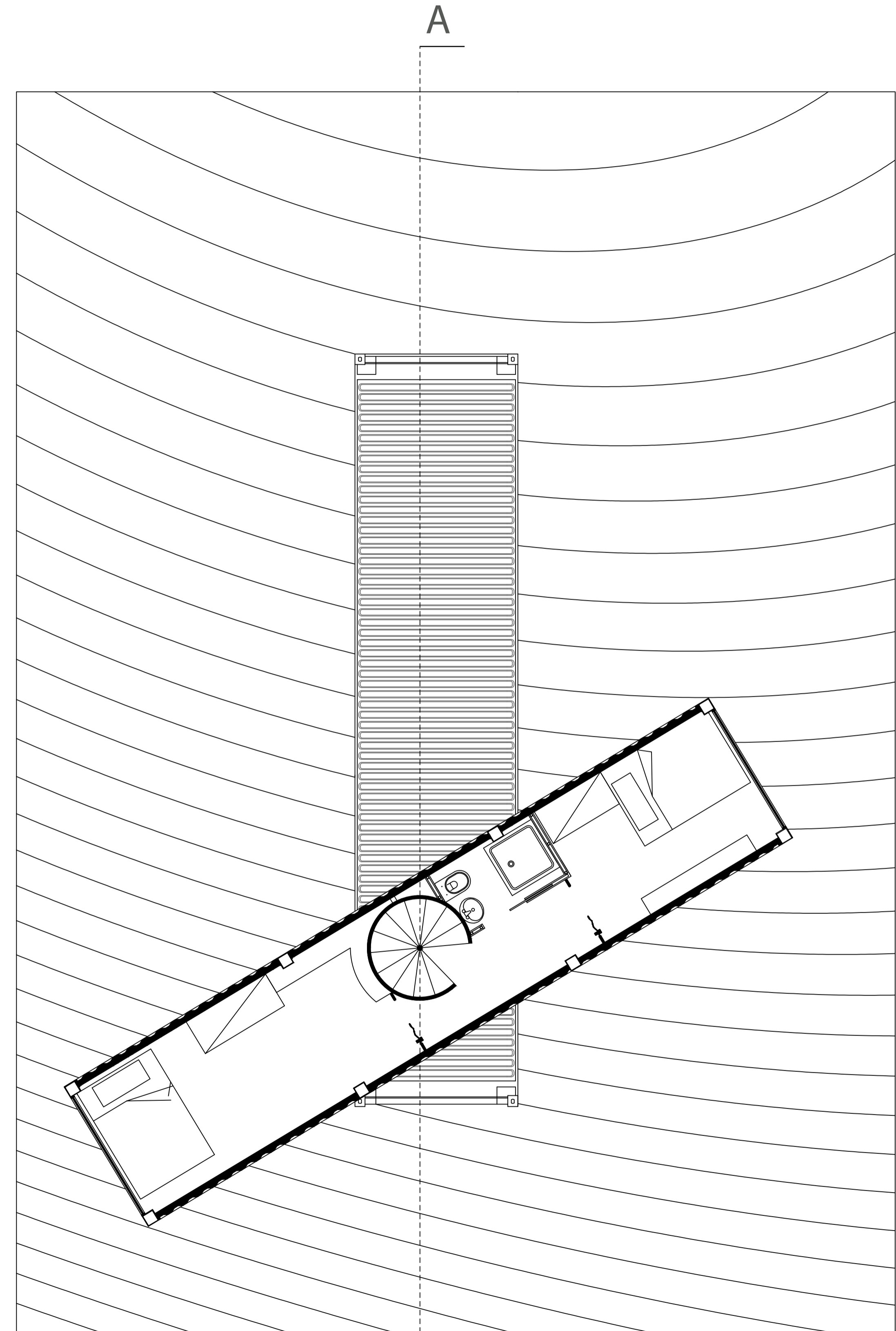
Second floor plan 1 : 50
